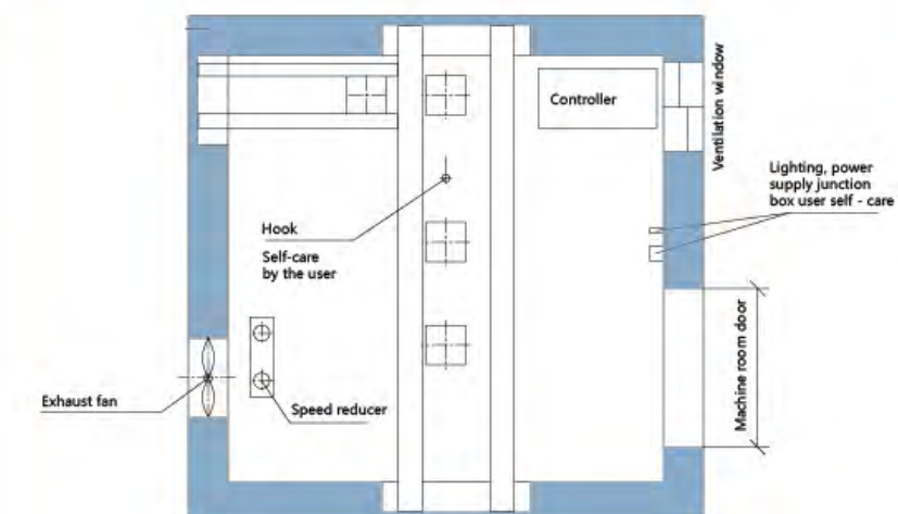
Machine room plane layout
