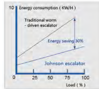
Helical gear reducer than worm gear Efficiency diagram of the auxiliary reducer
