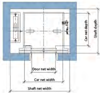
Shaft plan layout
