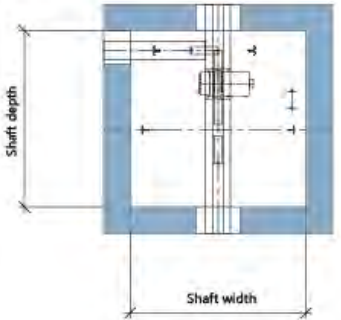
Shaft top plan layout
