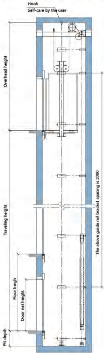
Rotation shaft vertical section
