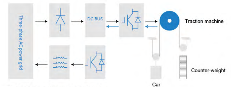
Working diagram of energy feedback system
