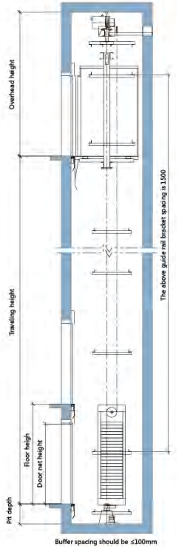
Rotation shaft vertical section
