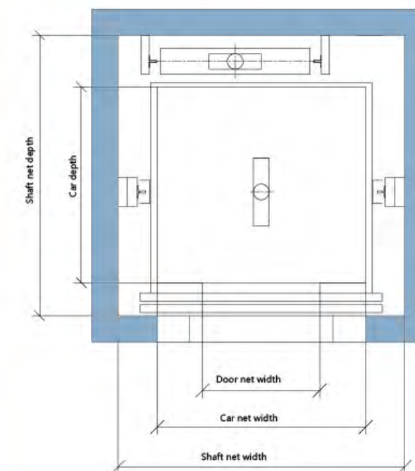
Shaft plan layout
