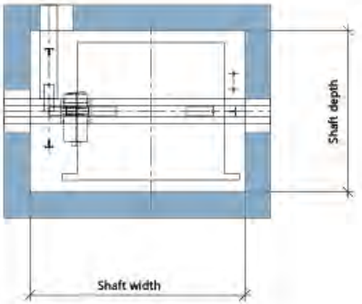
Shaft top plan layout
